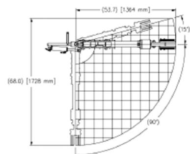
Plan View 1 Square = 5 inches (127 mm)
