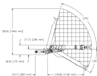
Elevation View 1 Square = 5 inches (127mm)
