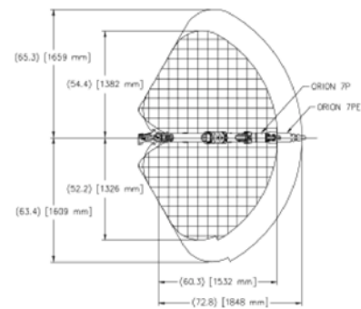
Plan View 1 Square = 5 inches (127 mm)
