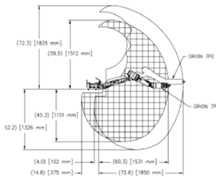
Elevation View 1 Square = 5 inches (127 mm)
