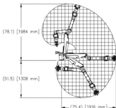
Elevation View 1 Square = 5 inches (127 mm)
