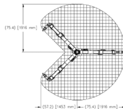
Plan View 1 Square = 5 inches (127 mm)
